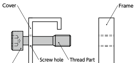
SSC(INCH) Socket Head Cap Captive Screw (Inch Screws)
