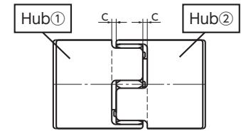
Fig. 3 Clearance C between hubs
